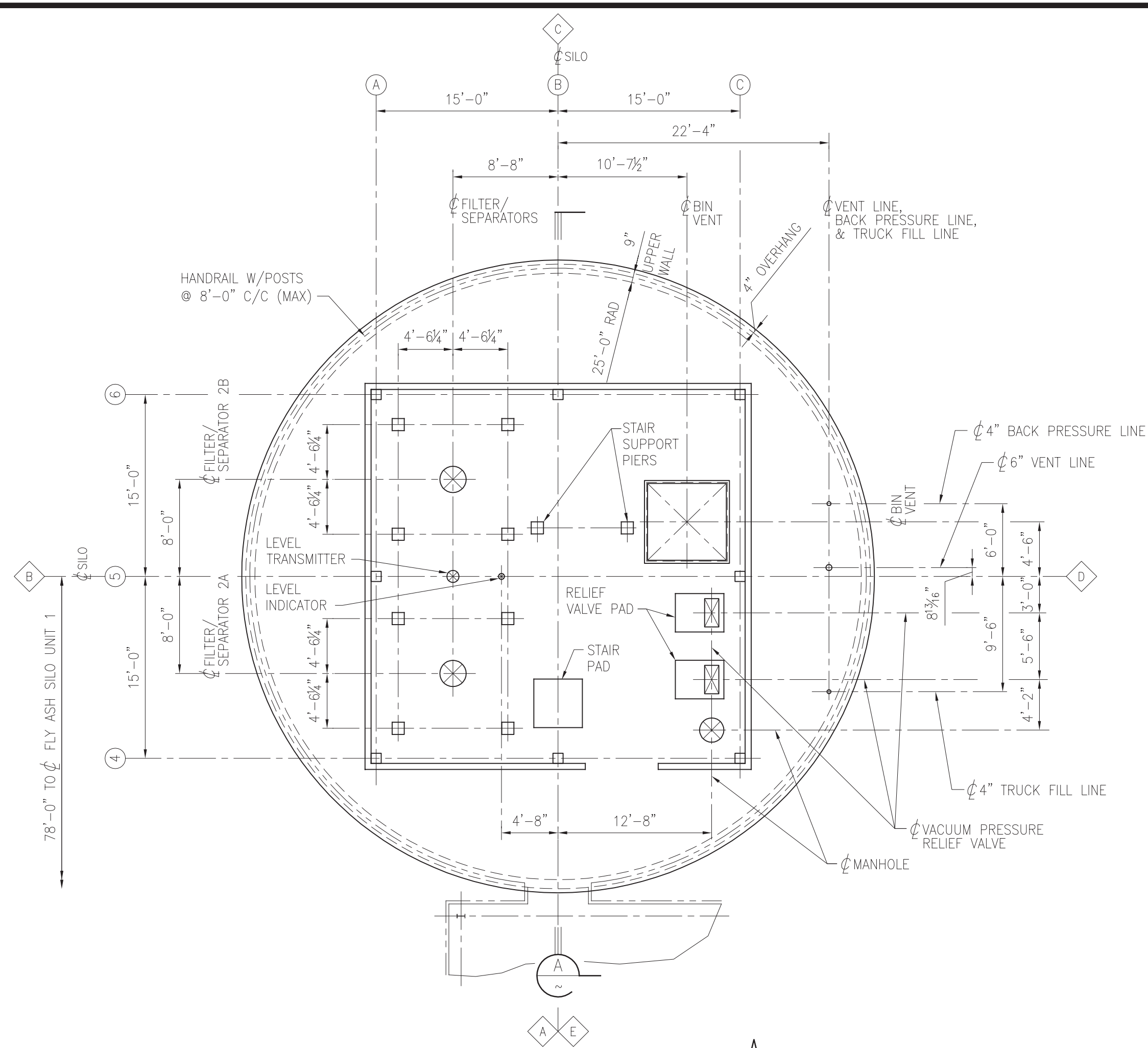
ROOF PLAN \frac{1}{8}''=1'-0'' T/WALL EL 687'-8 1/2"
