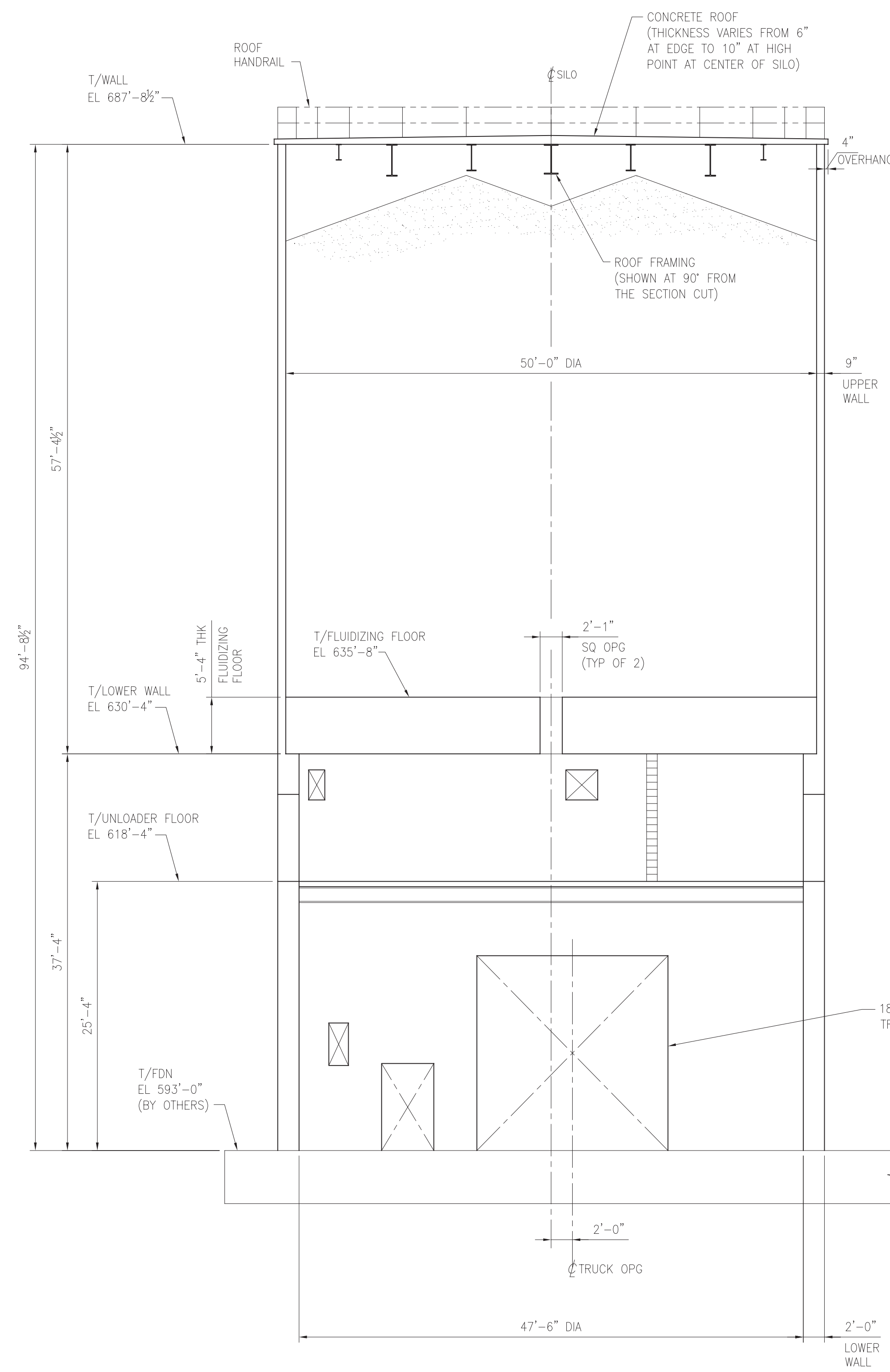
A TYPICAL SECTION THRU SILO \frac{1}{8}''=1'-0'' (LOOKING EAST)
