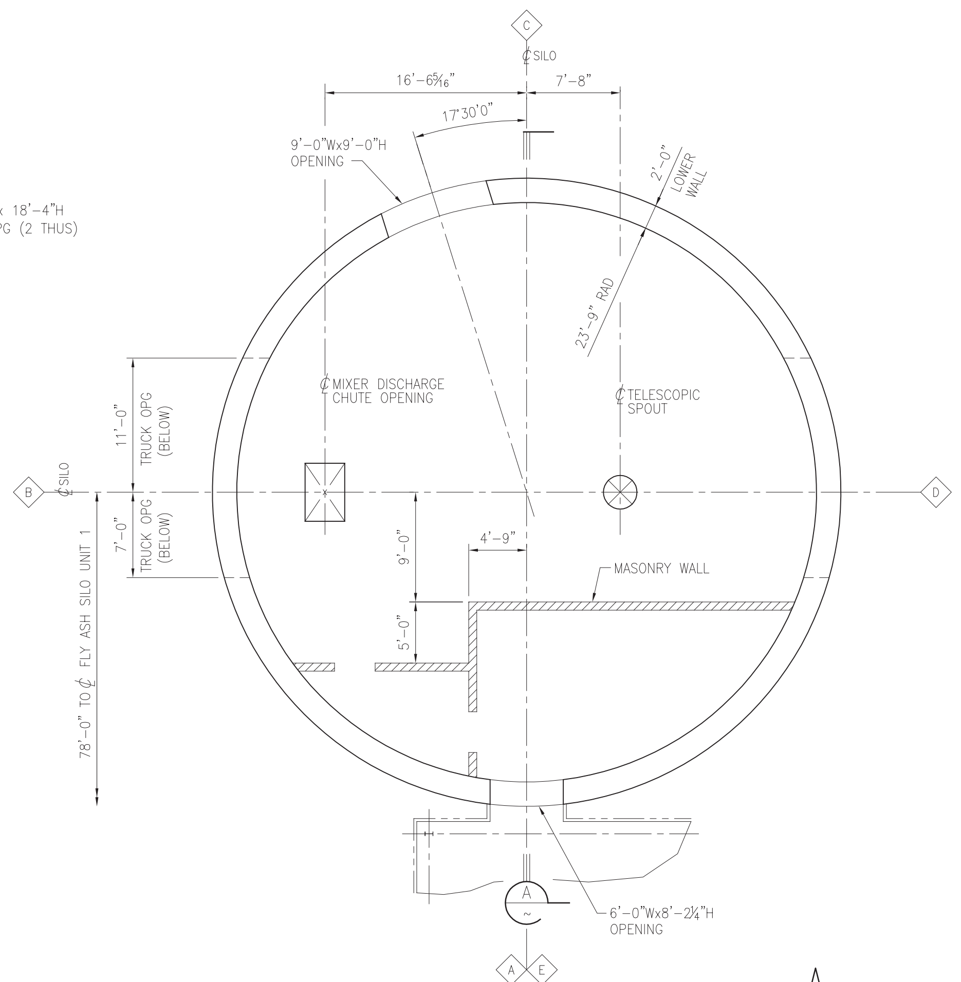
PLAN @ T/UNLOADER FLOOR \frac{1}{8}''=1'-0'' T/UNLOADER FLOOR EL 618'-4"
