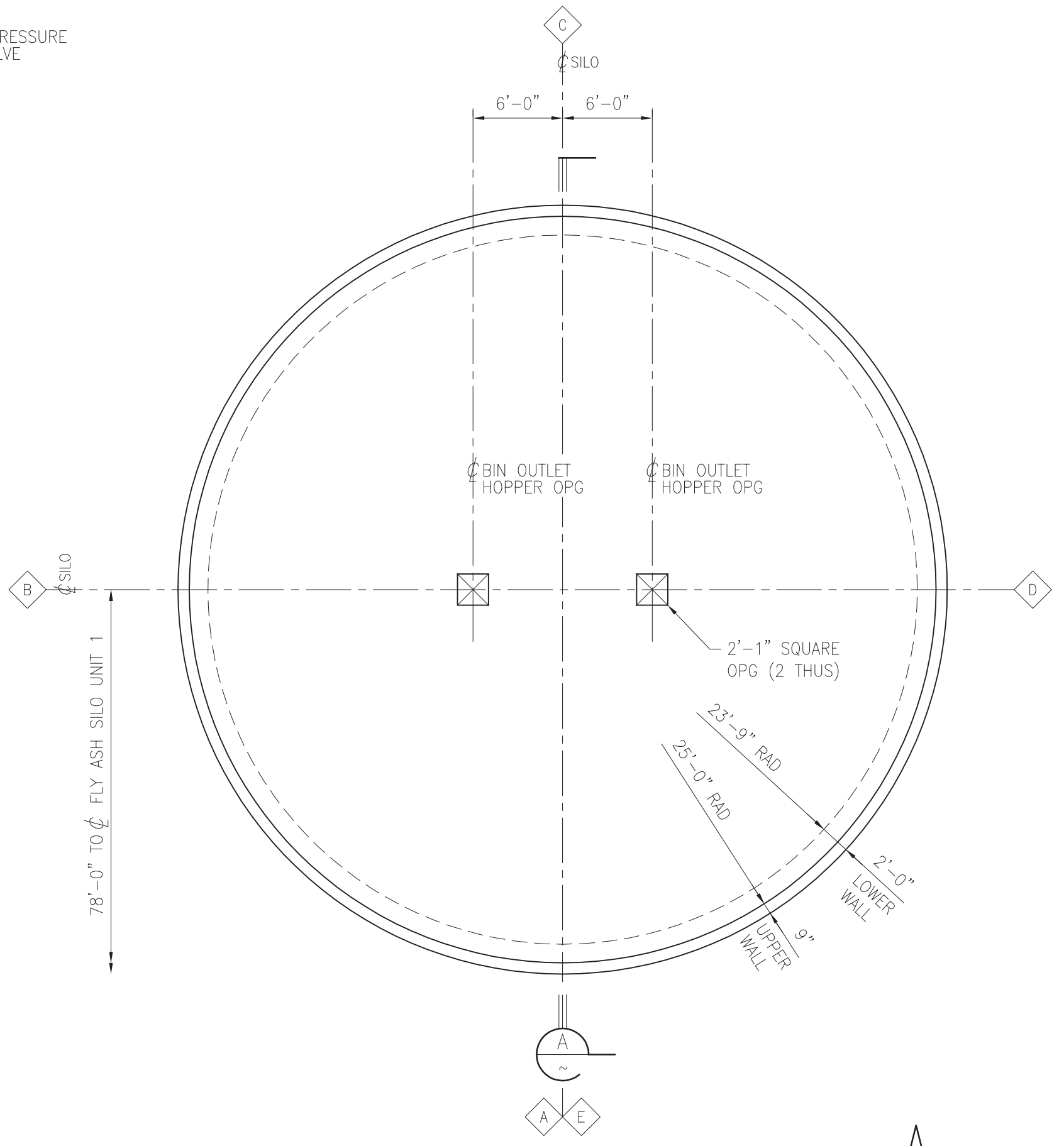
PLAN @ T/FLUIDIZING FLOOR \frac{1}{8}''=1'-0'' T/FLUIDIZING FLOOR EL 635'-8" FLUIDIZER ASSEMBLY PIPE SLEEVES NOT SHOWN FOR CLARITY
